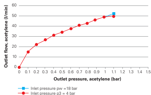
Regulationcurve 618-VIPR valve (Acetylene gas)
