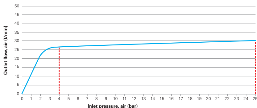
Regulationcurve 618-VIPR valve (Acetylene gas)
