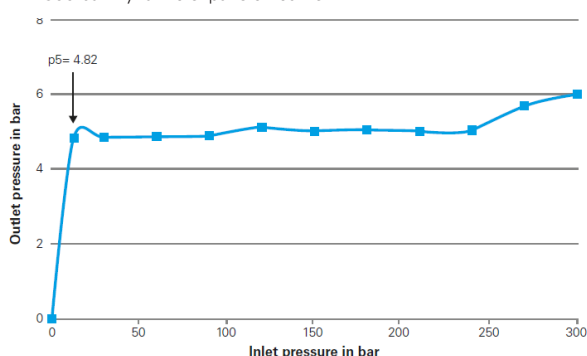
VIPR for Oxygen type "617" for inlet pressure 300 bar Dynamic expansion curve
