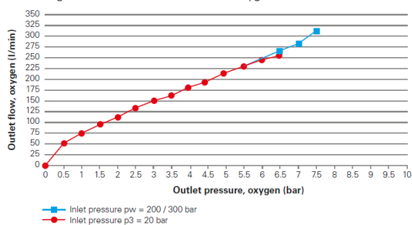
Regulation curve 617-VIPR Valve (Oxygen)
