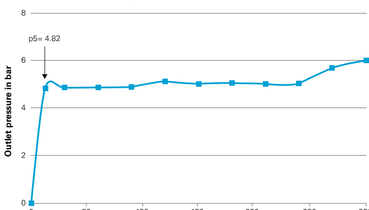
VIPR for Oxygen type "618" for inlet pressure 300 bar Dynamic expansion curve
